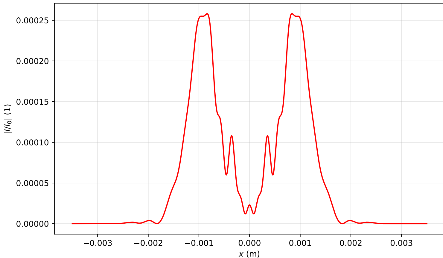
Intensity profile I(x, y = 0, z = 1.353)/I_0 , P_{in}=6.0P_{cr} , artificial time
